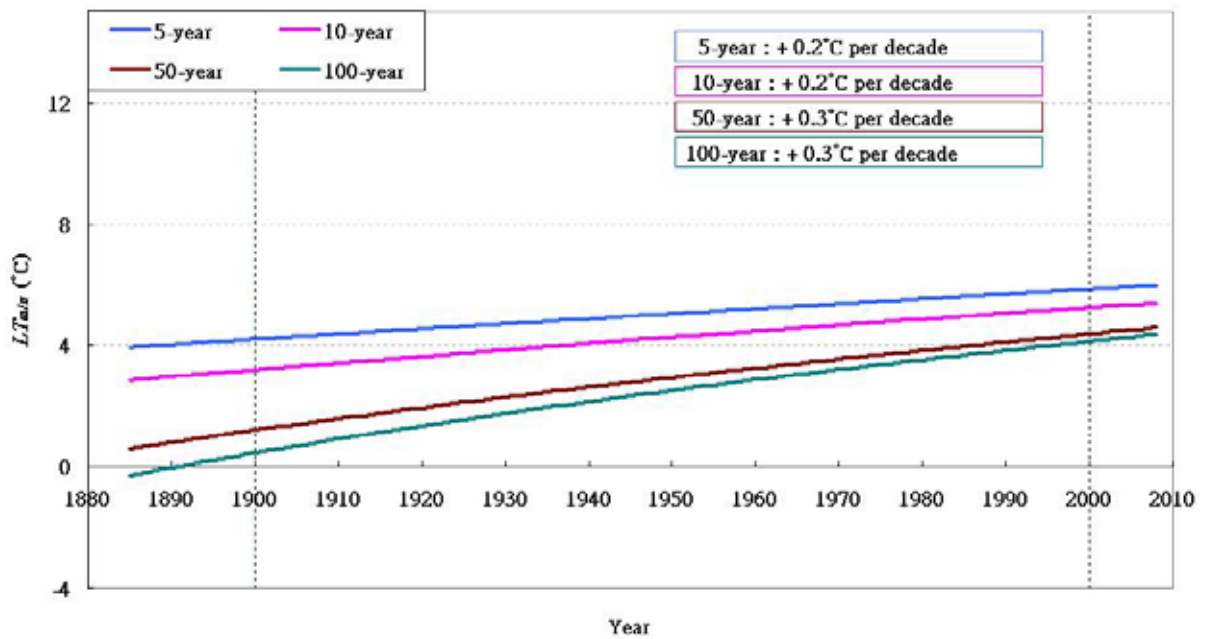
Figure 1.3(a). Long term trends of the return values for LT_{min} with return periods of 5-year, 10-year, 50-year and 100-year respectively (1885-2008)
