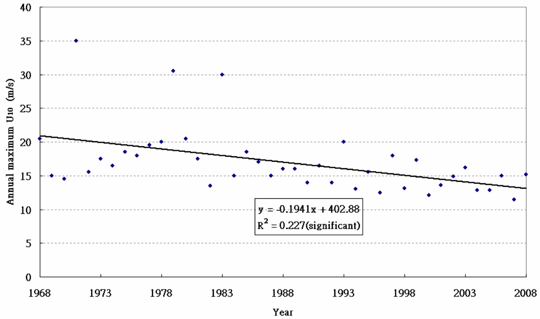
Figure 3.2(c). Time series of the annual maximum U_{10} at Kai Tak (1968-2008)
