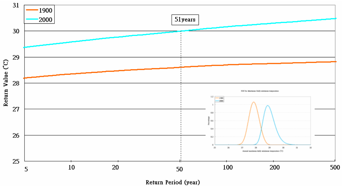
Figure 1.4(b). Return periods for HT_{min} in 1900 and 2000 (the insert shows the GEV pdf for HT_{min} in 1900 [brown line] and 2000 [blue line])
