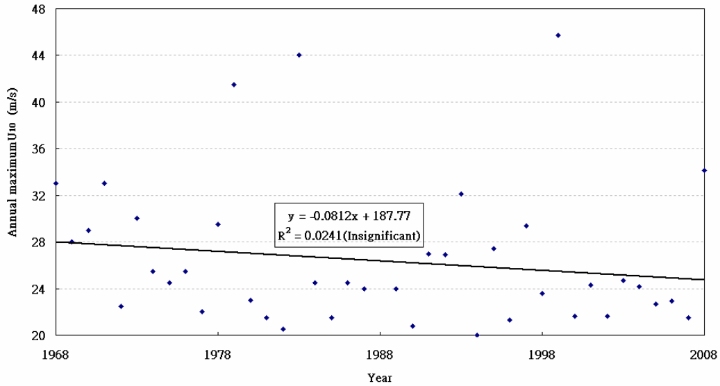
Figure 3.2(a). Time series of annual maximum U_{10} at Waglan Island (1968-2008)
