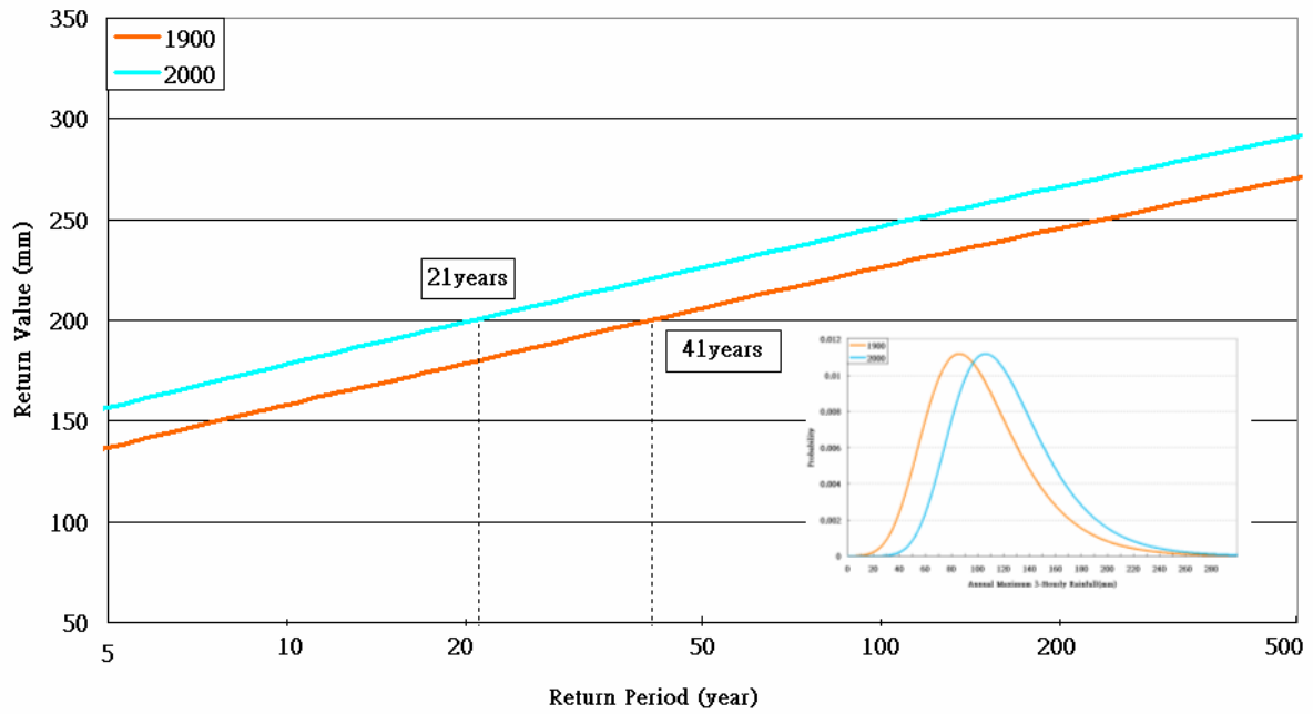
Figure 2.4(c). Return periods for annual maximum three-hourly rainfalls in 1900 and 2000 (the insert shows the GEV pdf for annual maximum three-hourly rainfalls in 1900 [brown line] and 2000 [blue line])
