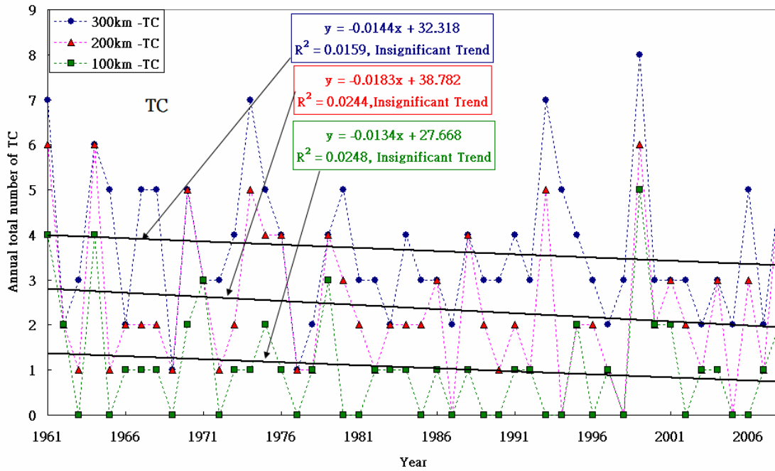
Figure 3.1(a). Time series of the annual number of tropical cyclones of any intensity passing within 100, 200 and 300 km of Hong Kong (1961-2008)
