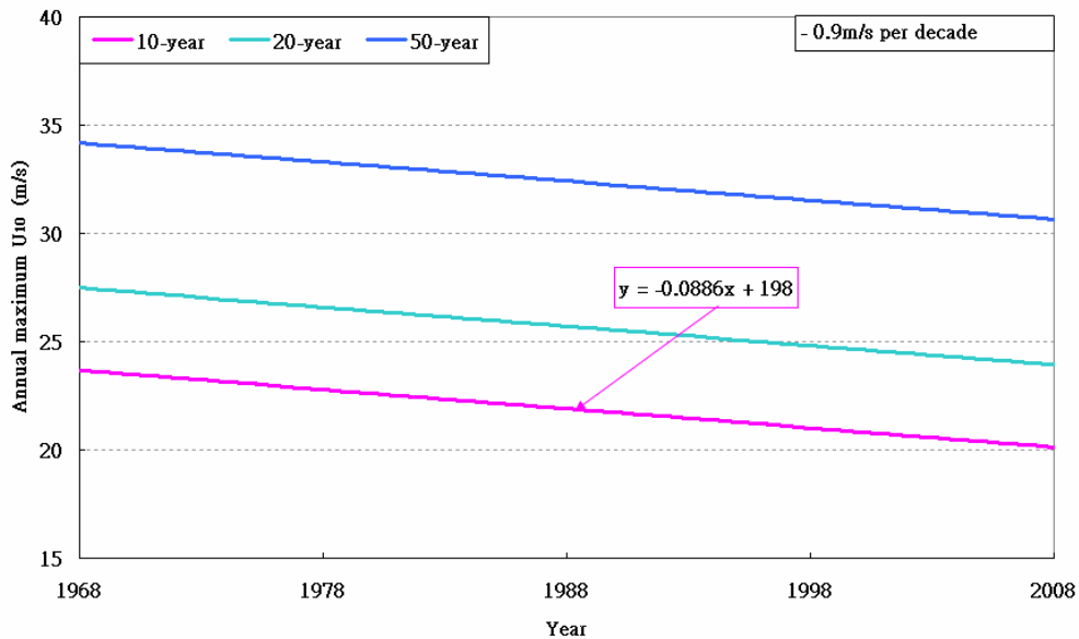
Figure 3.3(a). Long term trends of return values for the annual maximum U_{10} at Kai Tak with return periods of 10-year, 20-year and 50-year respectively (1968-2008)
