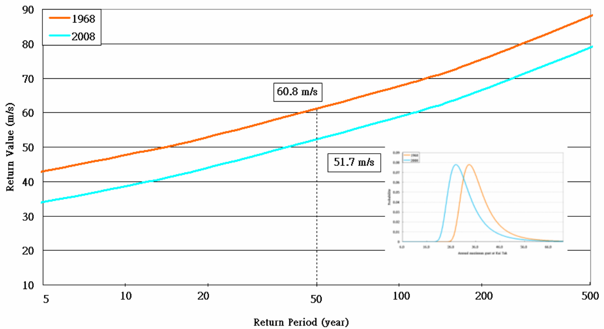
Figure 3.4(d). Return values for annual maximum U_g at Kai Tak in 1968 and 2008 (the insert shows the GEV pdf for annual maximum U_g at Kai Tak in 1968 [brown line] and 2008 [blue line])
