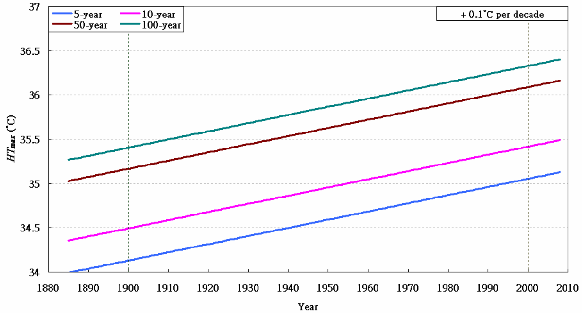
Figure 1.3(d). Long term trends of the return values for HT_{max} with return periods of 5-year, 10-year, 50-year and 100-year respectively (1885-2008)
