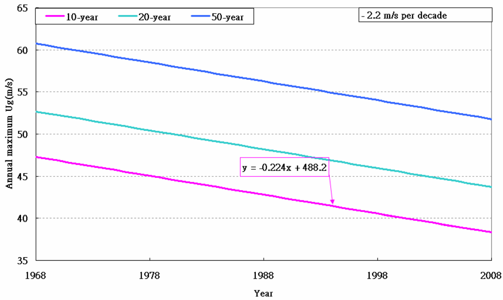
Figure 3.3(b). Long term trends of the return values for the annual maximum U_g at Kai Tak with return periods of 10-year, 20-year and 50-year respectively (1968-2008)
