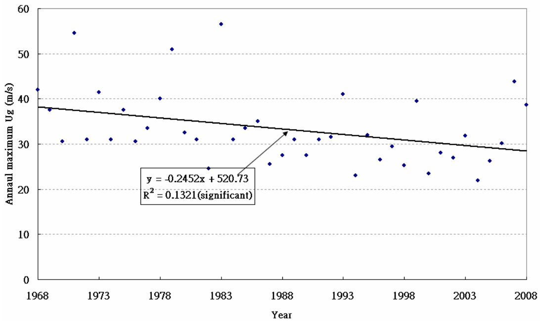
Figure 3.2(d). Time series of annual maximum U_g at Kai Tak (1968-2008)
