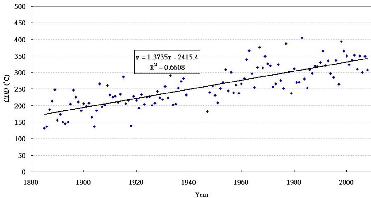
Figure 1.5(b). Time series of Cooling Degree-Day (1885-2008)
