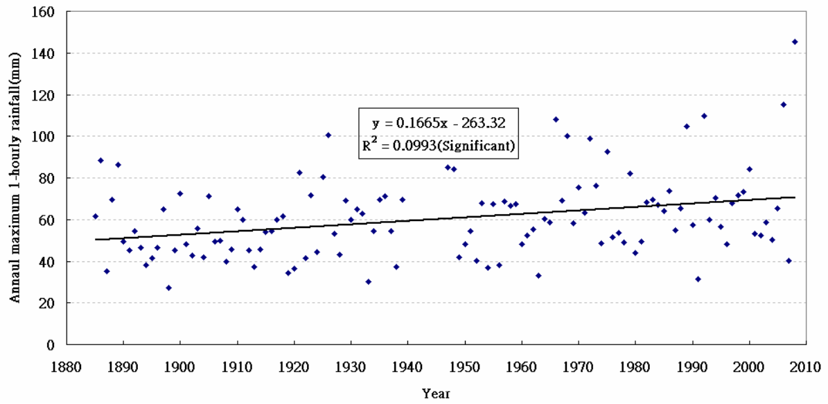
Figure 2.2(a). Time series of annual maximum 1-hourly rainfall (1885-2008)
