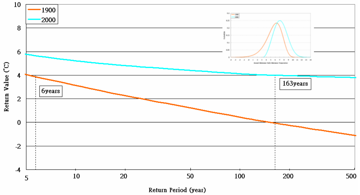
Figure 1.4(a). Return periods for LT_{min} in 1900 and 2000 (the insert shows the GEV pdf for LT_{min} in 1900 [brown line] and 2000 [blue line])
