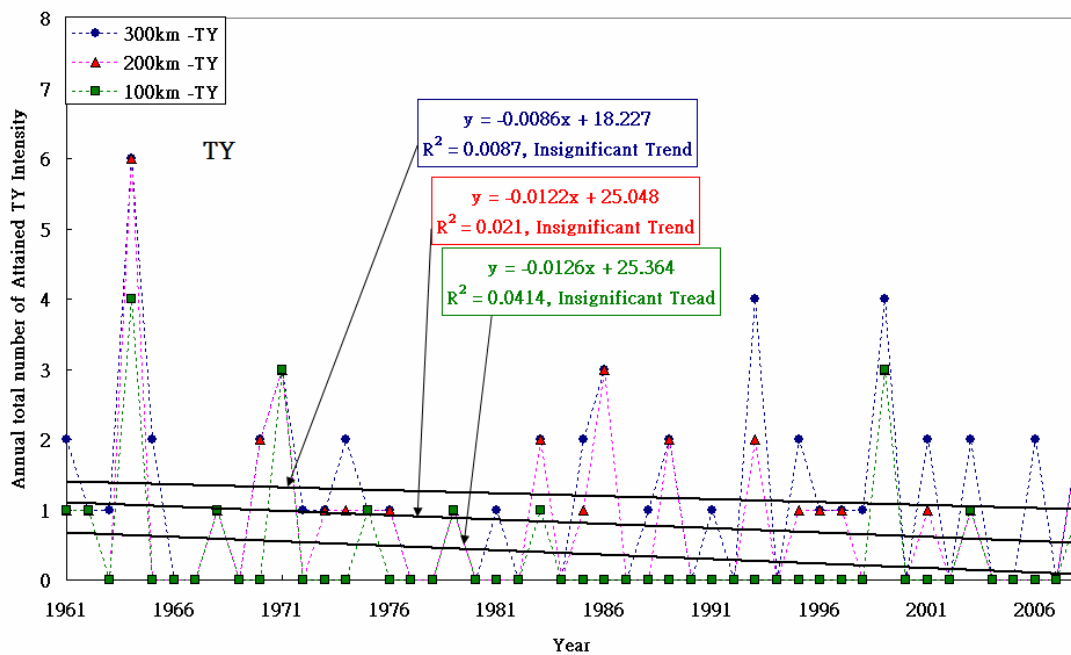
Figure 3.1(b). Time series of the annual number of typhoons passing within 100, 200 and 300 km of Hong Kong (1961-2008)
