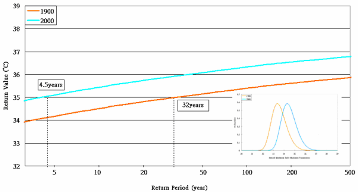
Figure 1.4(d). Return periods for HT_{max} in 1900 and 2000 (the insert shows the GEV pdf for HT_{max} in 1900 [brown line] and 2000 [blue line])
