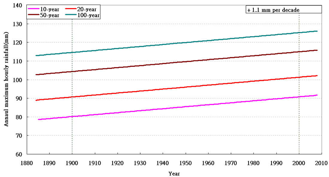
Figure 2.3(a). Long term trends of the return values for the annual maximum one-hourly rainfall with return periods of 10-year, 20-year, 50-year and 100-year respectively (1885-2008)
