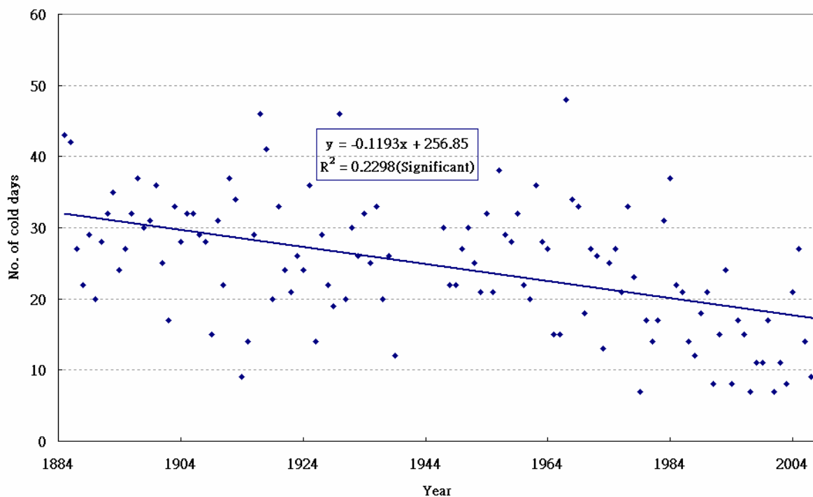
Figure 1.1(a). Annual number of cold days (1885-2008)
