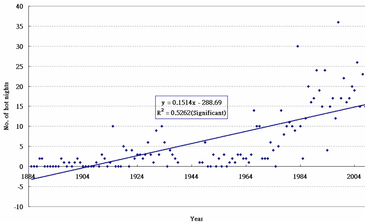
Figure 1.1(c). Annual number of hot nights (1885-2008)
