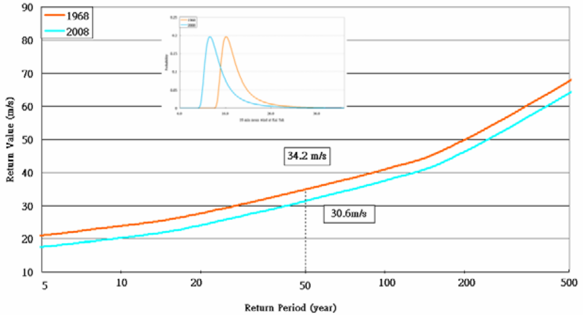
Figure 3.4(c). Return values for annual maximum U_{10} at Kai Tak in 1968 and 2008 (the insert shows the GEV pdf for annual maximum U_{10} at Kai Tak in 1968 [brown line] and 2008 [blue line])
