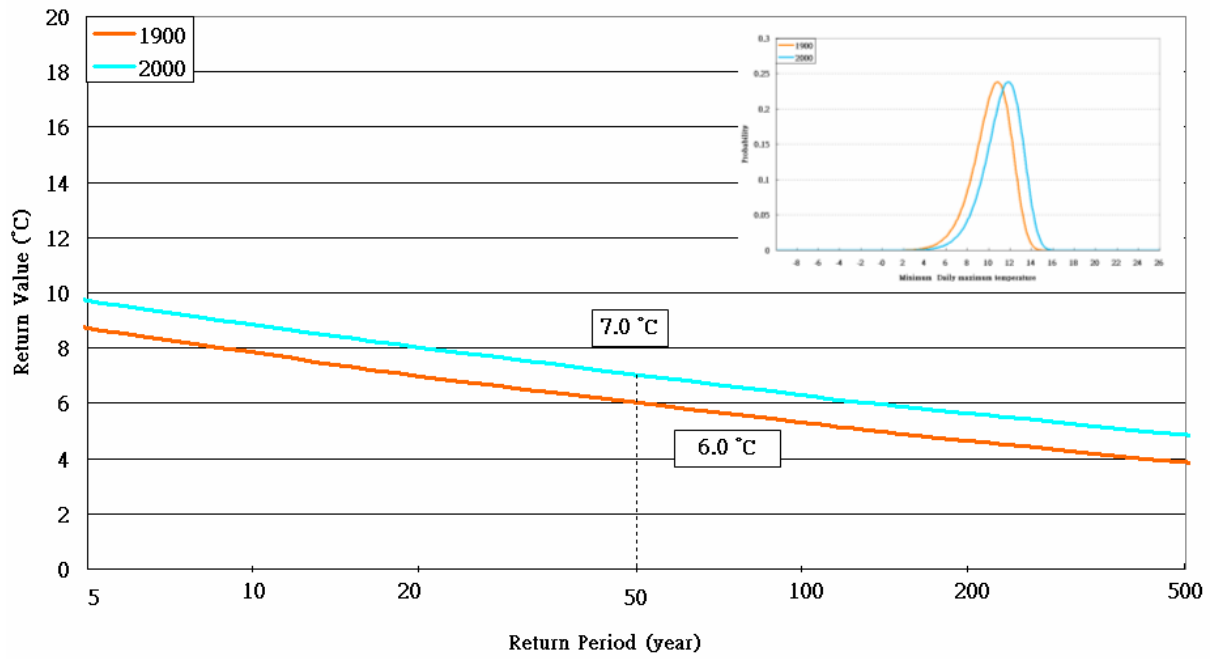
Figure 1.4(c). Return periods for LT_{max} in 1900 and 2000 (the insert shows the GEV pdf for LT_{max} in 1900 [brown line] and 2000 [blue line])
