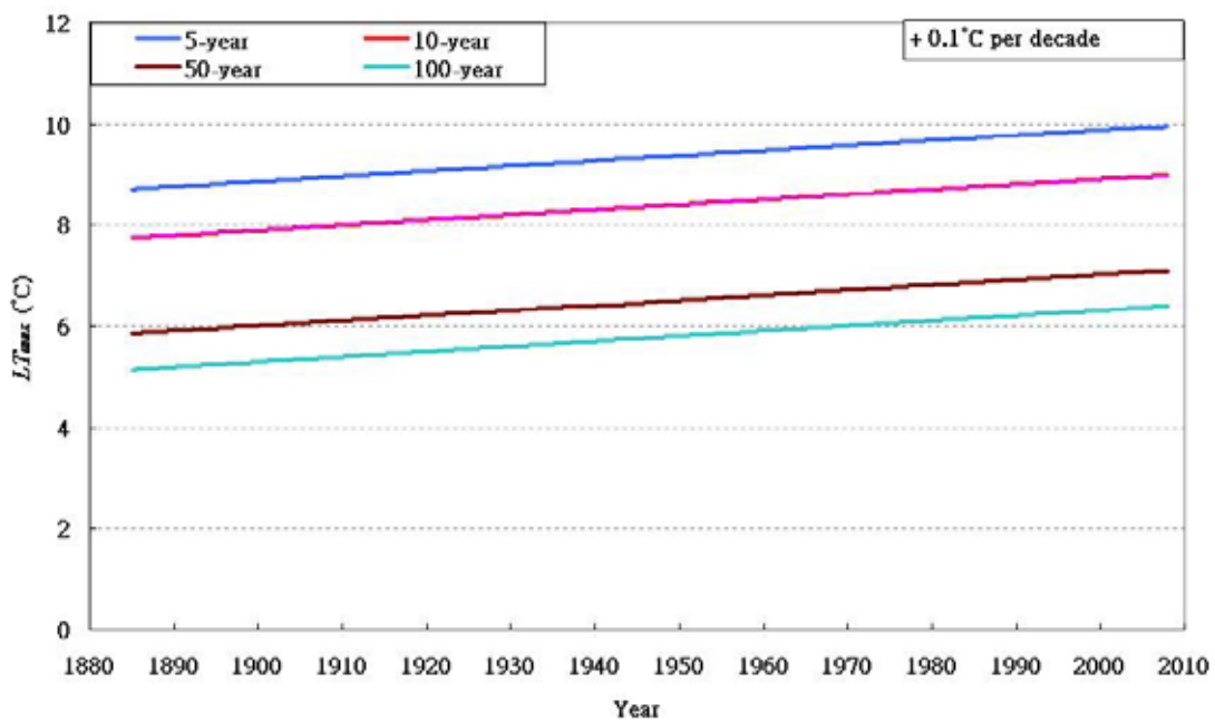
Figure 1.3(c). Long term trends of the return values for LT_{max} with return periods of 5-year, 10-year, 50-year and 100-year respectively (1885-2008)
