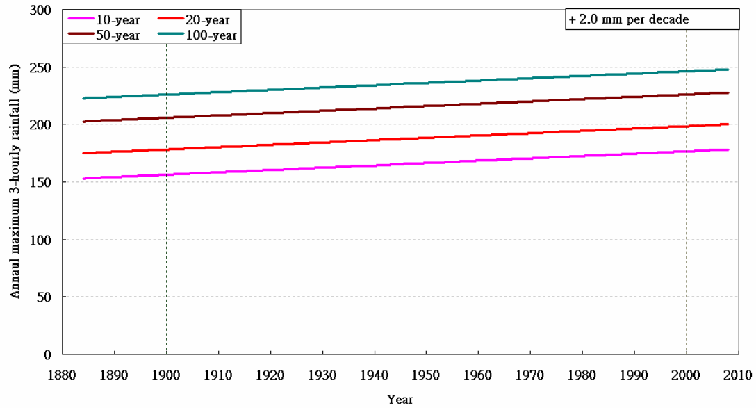
Figure 2.3(c). Long term trends of the return values for the annual maximum three-hourly rainfall with return periods of 10-year, 20-year, 50-year and 100-year respectively (1885-2008)
