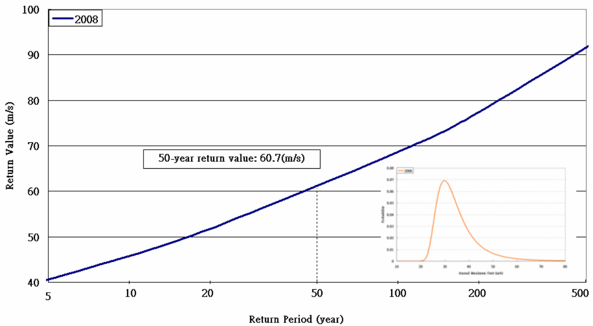
Figure 3.4(b). Return values for annual maximum U_g at Waglan Island in 2008 (the insert shows the GEV pdf for annual maximum U_g at Waglan Island in 2008)
