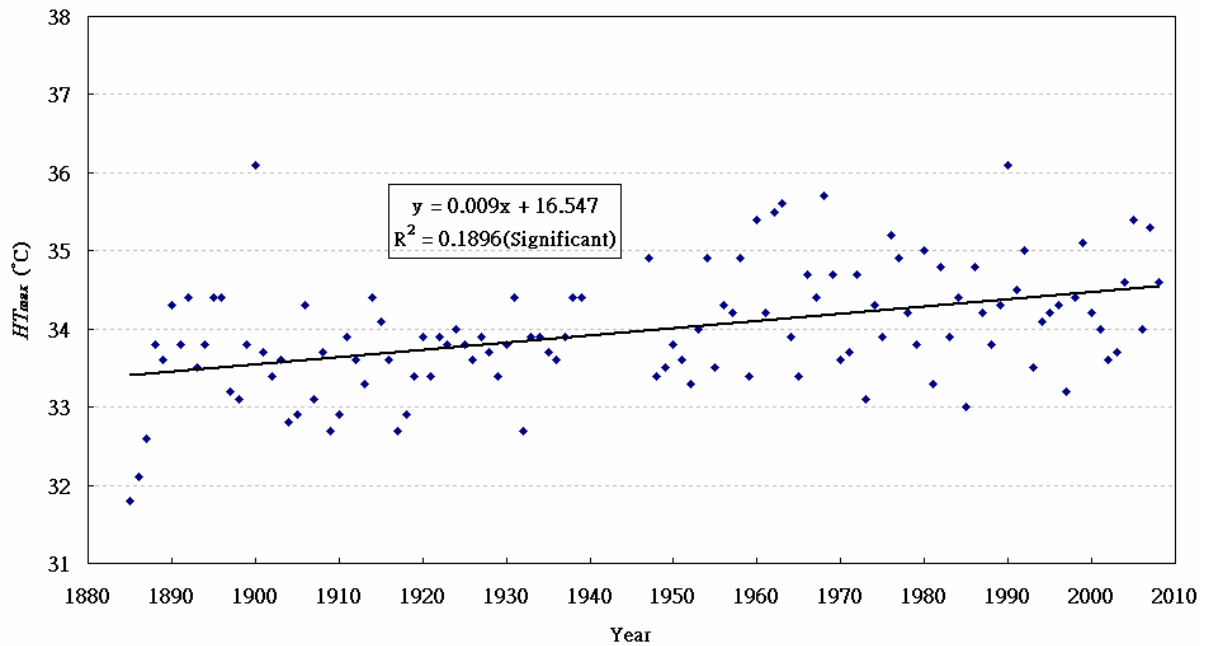
Figure 1.2(d). Time series of HT_{max} (1885-2008)
