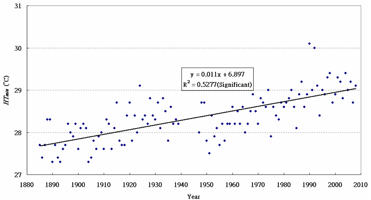
Figure 1.2(b). Time series of HT_{min} (1885-2008)
