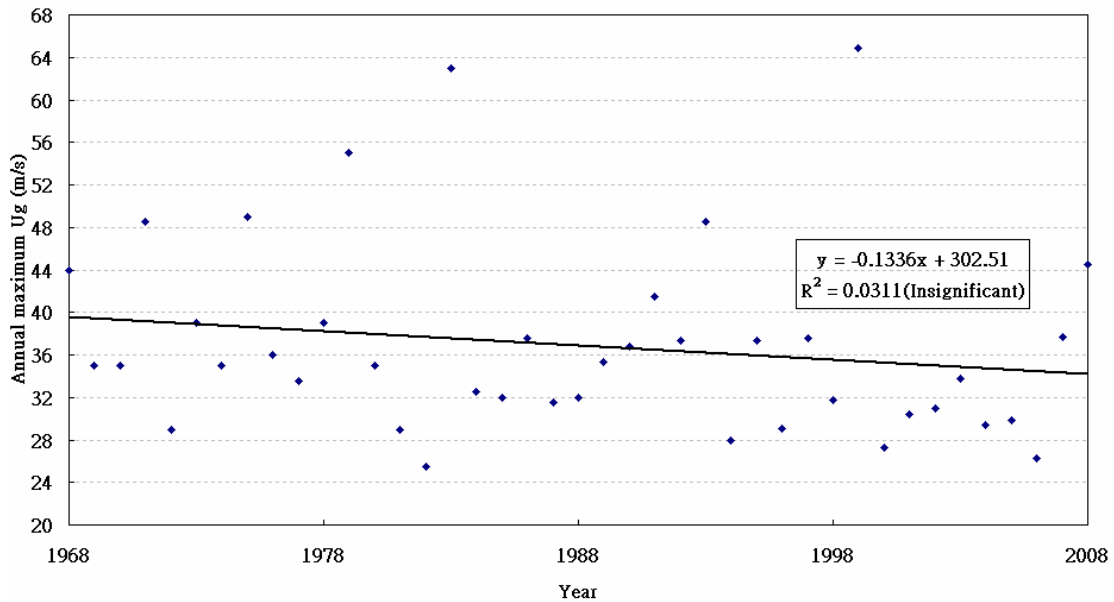
Figure 3.2(b). Time series of annual maximum U_g at Waglan Island (1968-2008)
