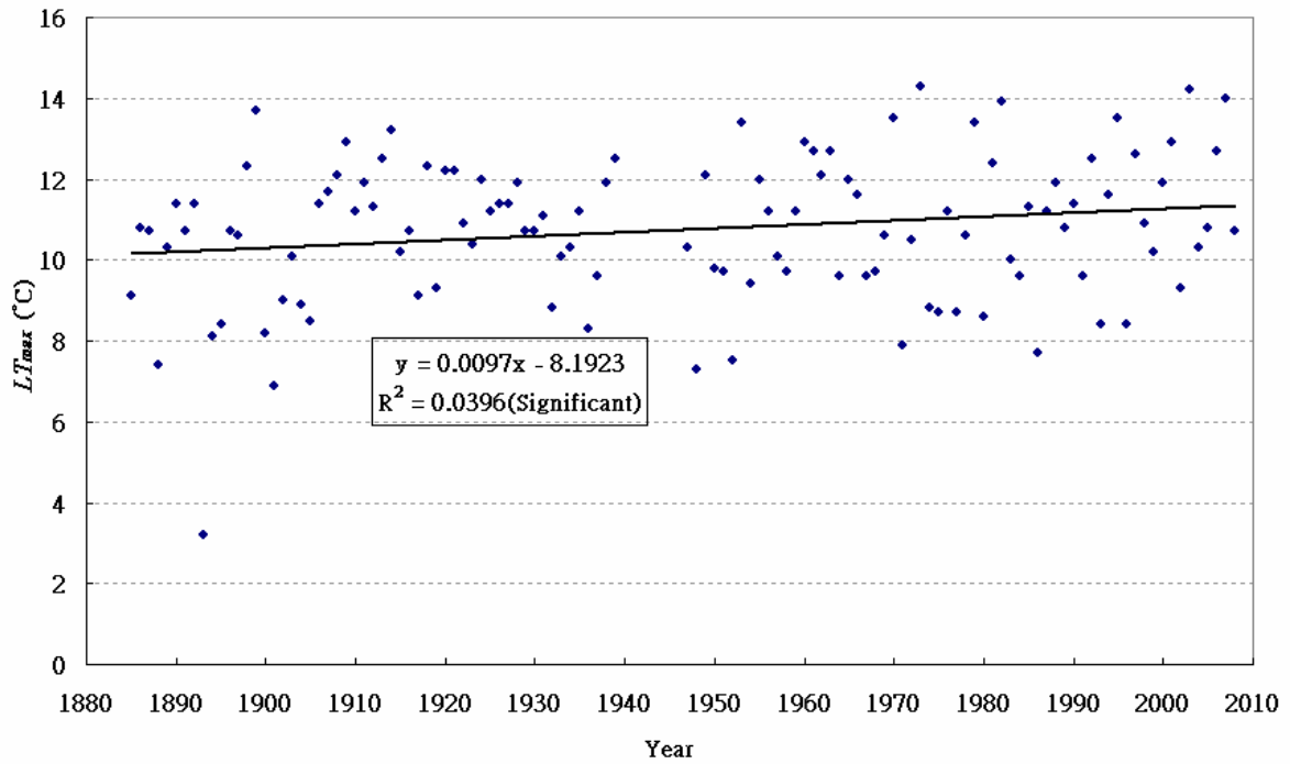
Figure 1.2(c). Time series of LT_{max} (1885-2008)
