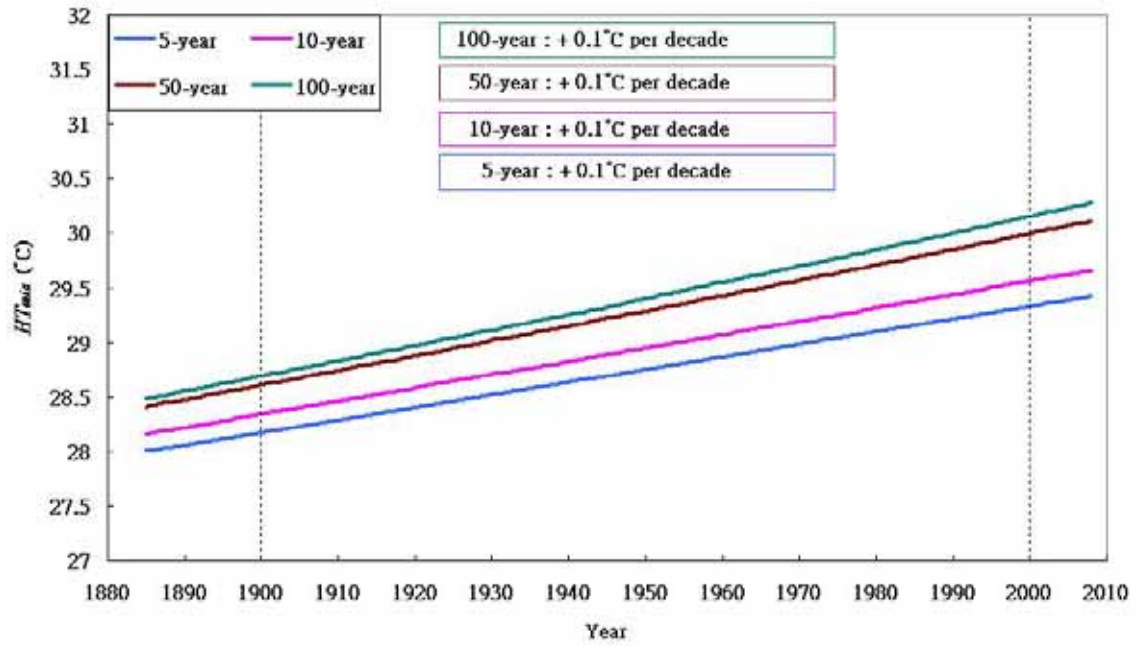
Figure 1.3(b). Long term trends of the return values for HT_{min} with return periods of 5-year, 10-year, 50-year and 100-year respectively (1885-2008)
