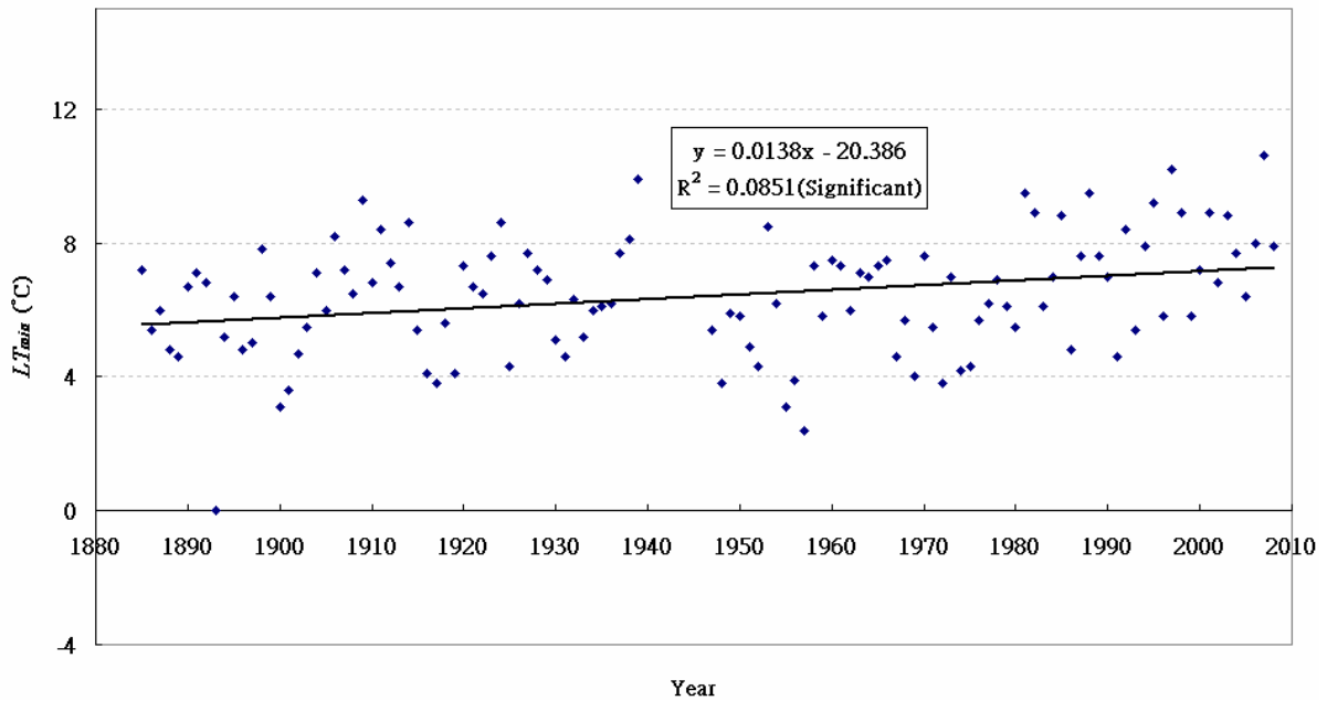
Figure 1.2(a). Time series of LT_{min} (1885-2008)
