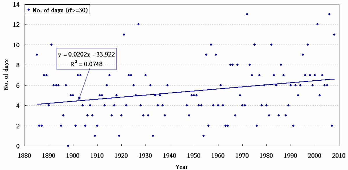
Figure 2.1. Annual number of days with an hourly rainfall exceeding 30 mm (1885-2008)
