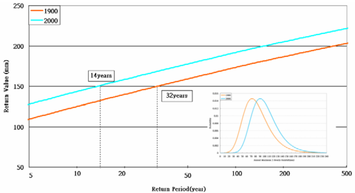
Figure 2.4(b). Return periods for annual maximum two-hourly rainfalls in 1900 and 2000 (the insert shows the GEV pdf for annual maximum two-hourly rainfalls in 1900 [brown line] and 2000 [blue line])
