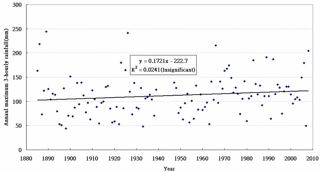
Figure 2.2(c). Time series of annual maximum 3-hourly rainfall (1885-2008)
