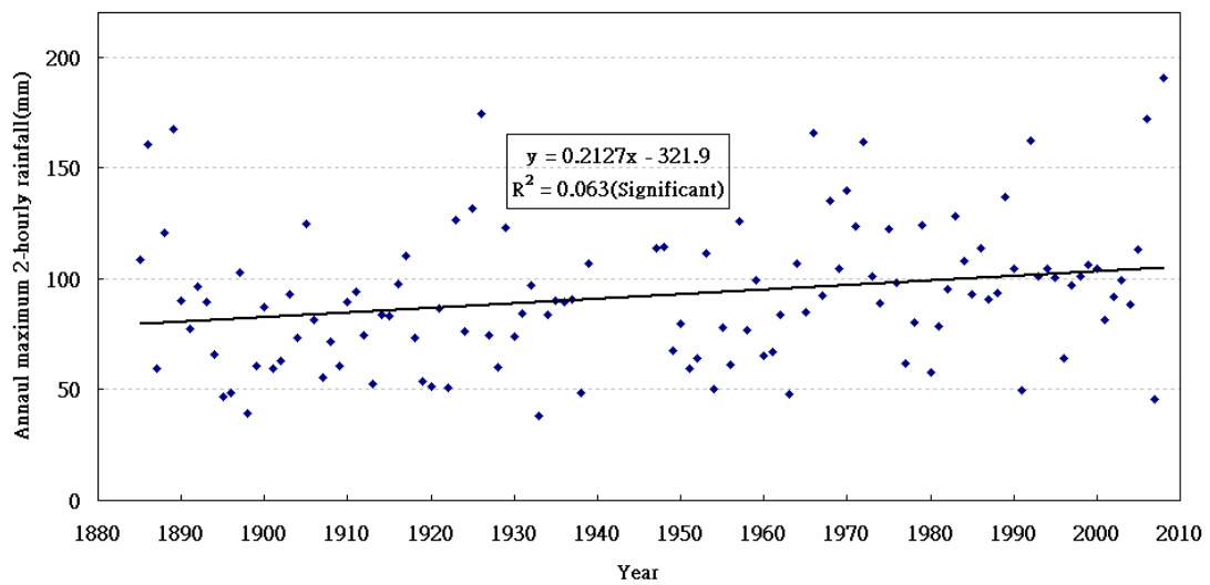
Figure 2.2(b). Time series of annual maximum 2-hourly rainfall (1885-2008)
