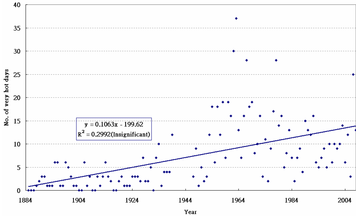
Figure 1.1(b). Annual number of very hot days (1885-2008)
