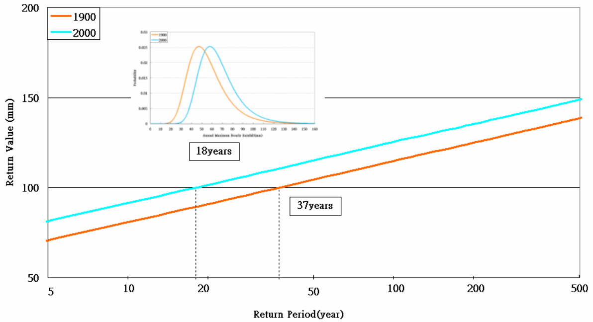
Figure 2.4(a). Return periods for annual maximum one-hourly rainfalls in 1900 and 2000 (the insert shows the GEV pdf for annual maximum one-hourly rainfalls in 1900 [brown line] and 2000 [blue line])
