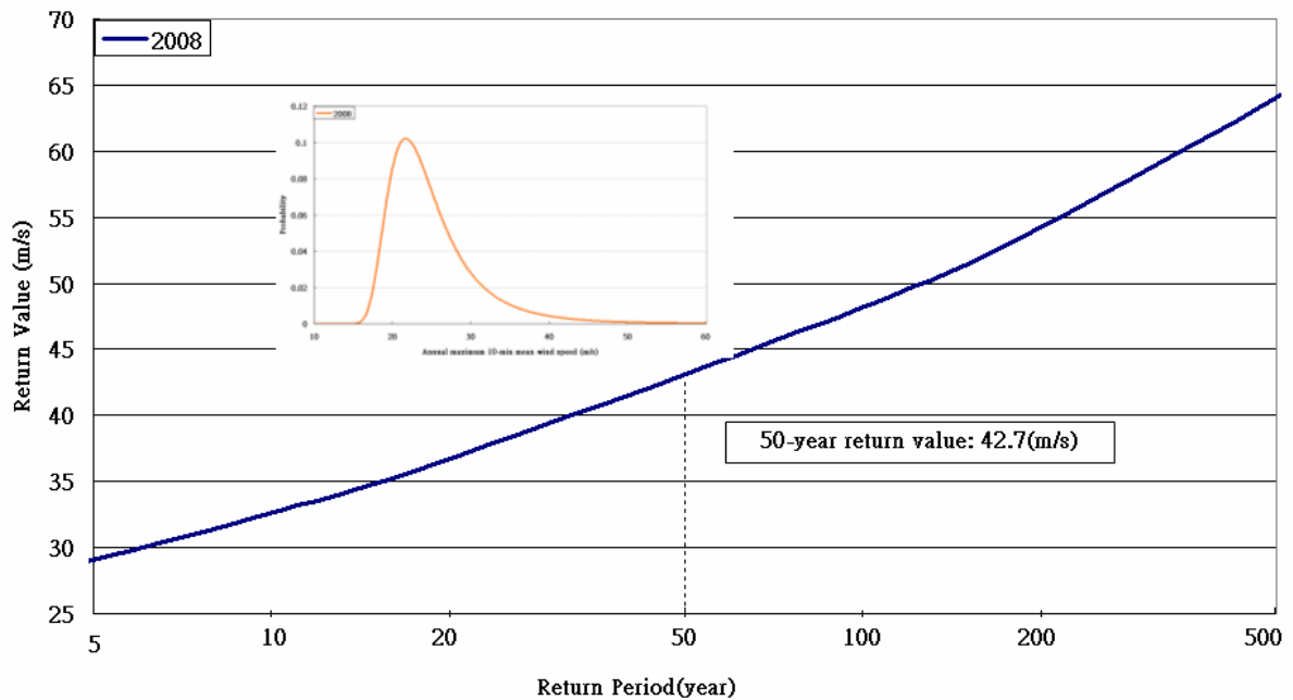
Figure 3.4(a). Return values for annual maximum U_{10} at Waglan Island in 2008 (the insert shows the GEV pdf for annual maximum U_{10} at Waglan Island in 2008)
