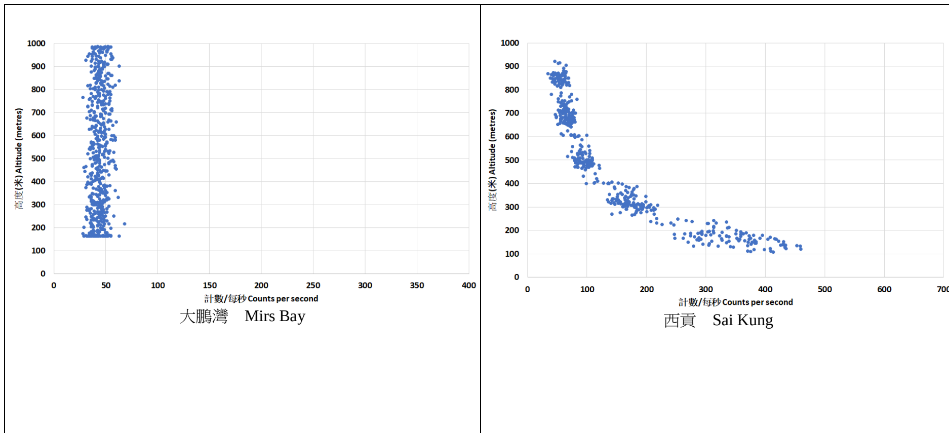
圖 5. 空中輻射監測系統在二零二二年七月十一日於大鵬灣海面及西貢上空測量的計數率隨高度的變化。 Figure 5. Variation of count rate with altitude over Mirs Bay and Sai Kung area, as measured by the Aerial Radiation Monitoring System on 11 July 2022.
