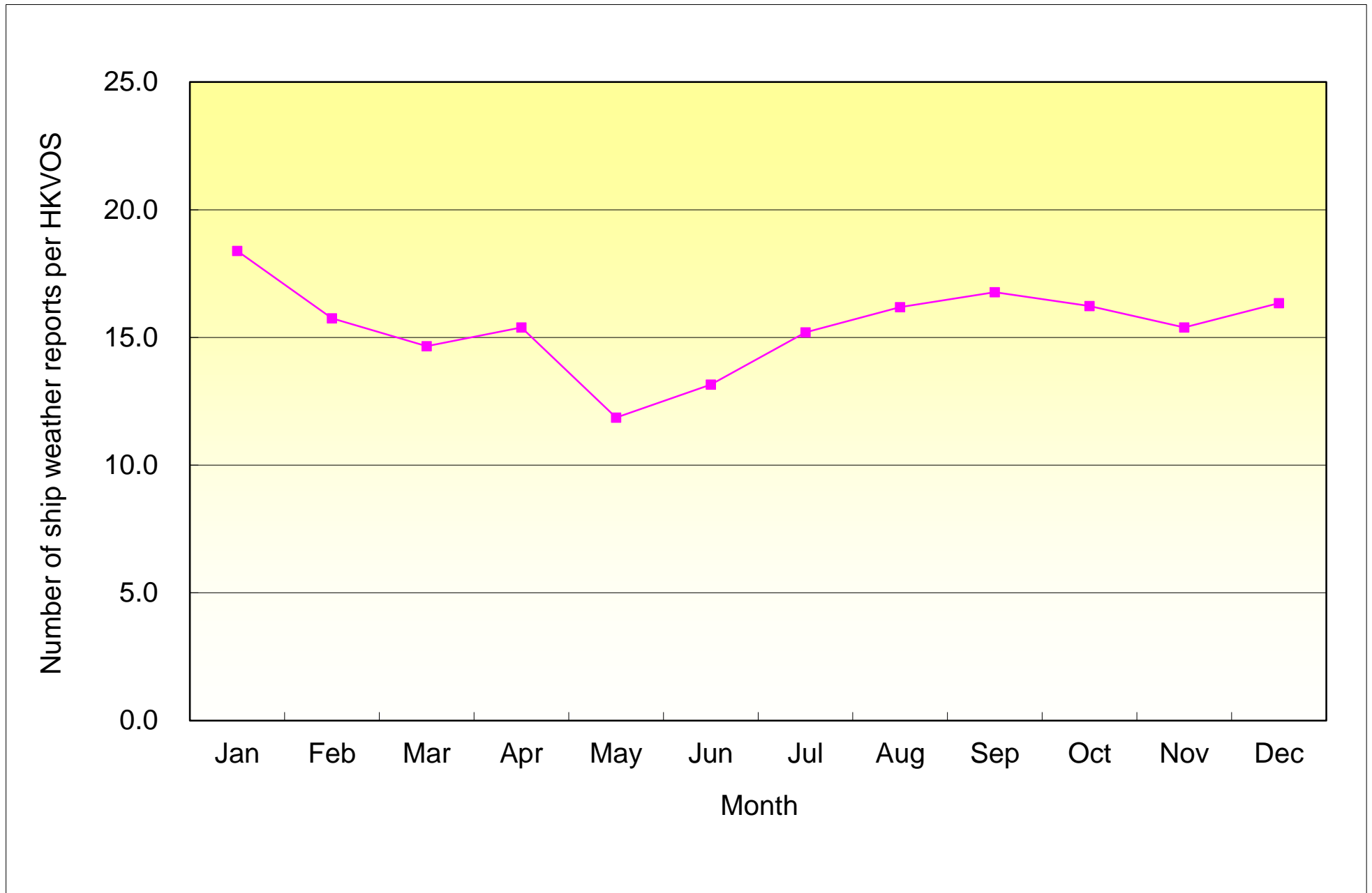
Number of ship weather reports per HKVOS in 2016
