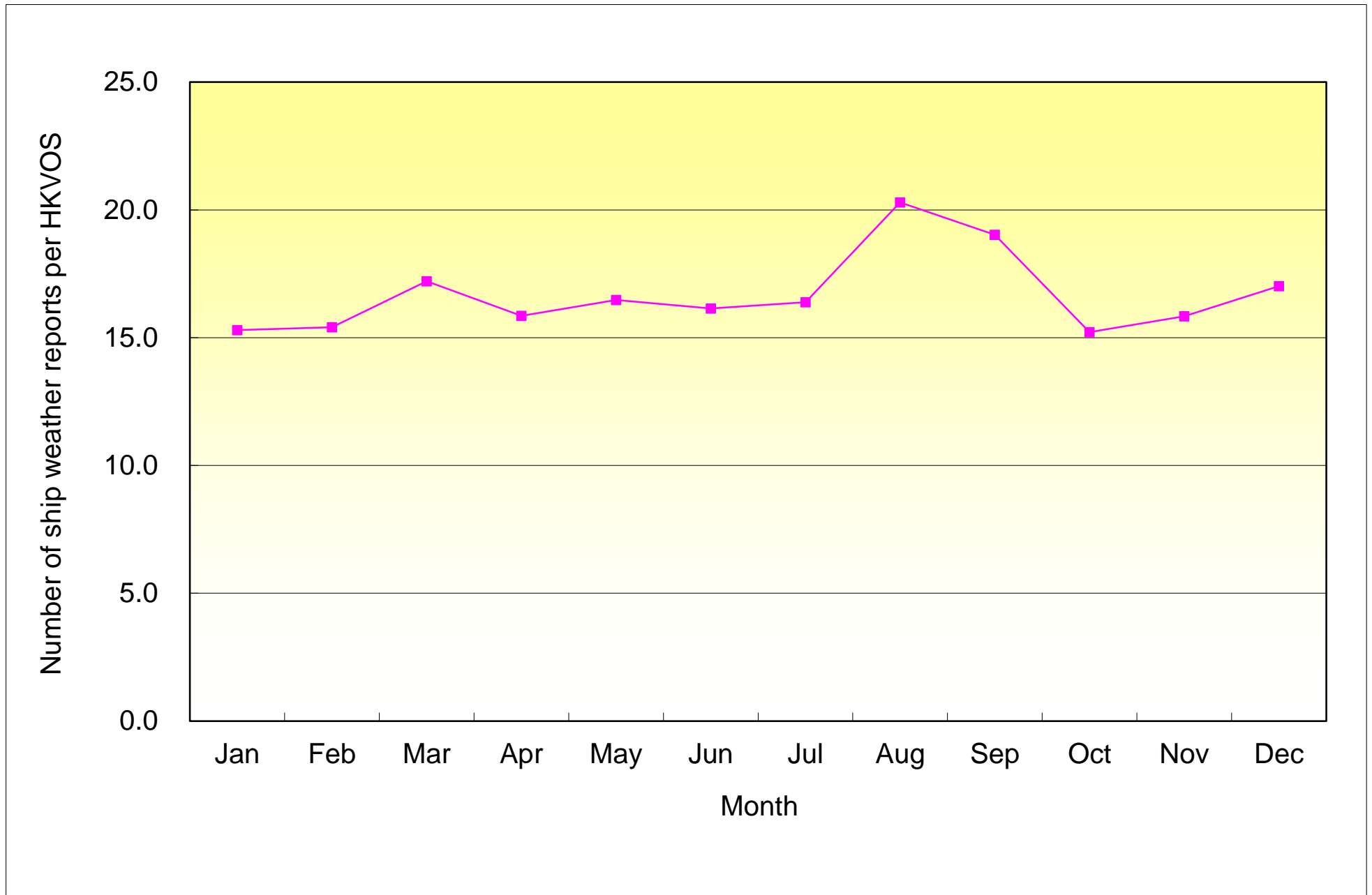
Number of ship weather reports per HKVOS in 2017
