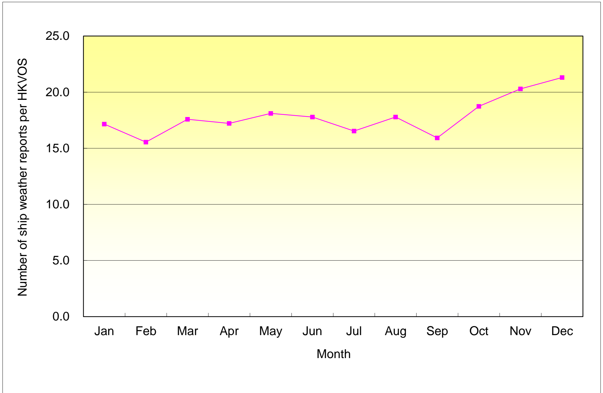
Number of ship weather reports per HKVOS in 2018
