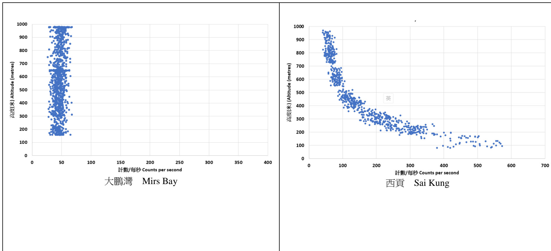
圖 5. 空中輻射監測系統在二零二一年七月十五日於大鵬灣海面及西貢上空測量的計數率隨高度的變化。 Figure 5. Variation of count rate with altitude over Mirs Bay and Sai Kung area, as measured by the Aerial Radiation Monitoring System on 15 July 2021.
