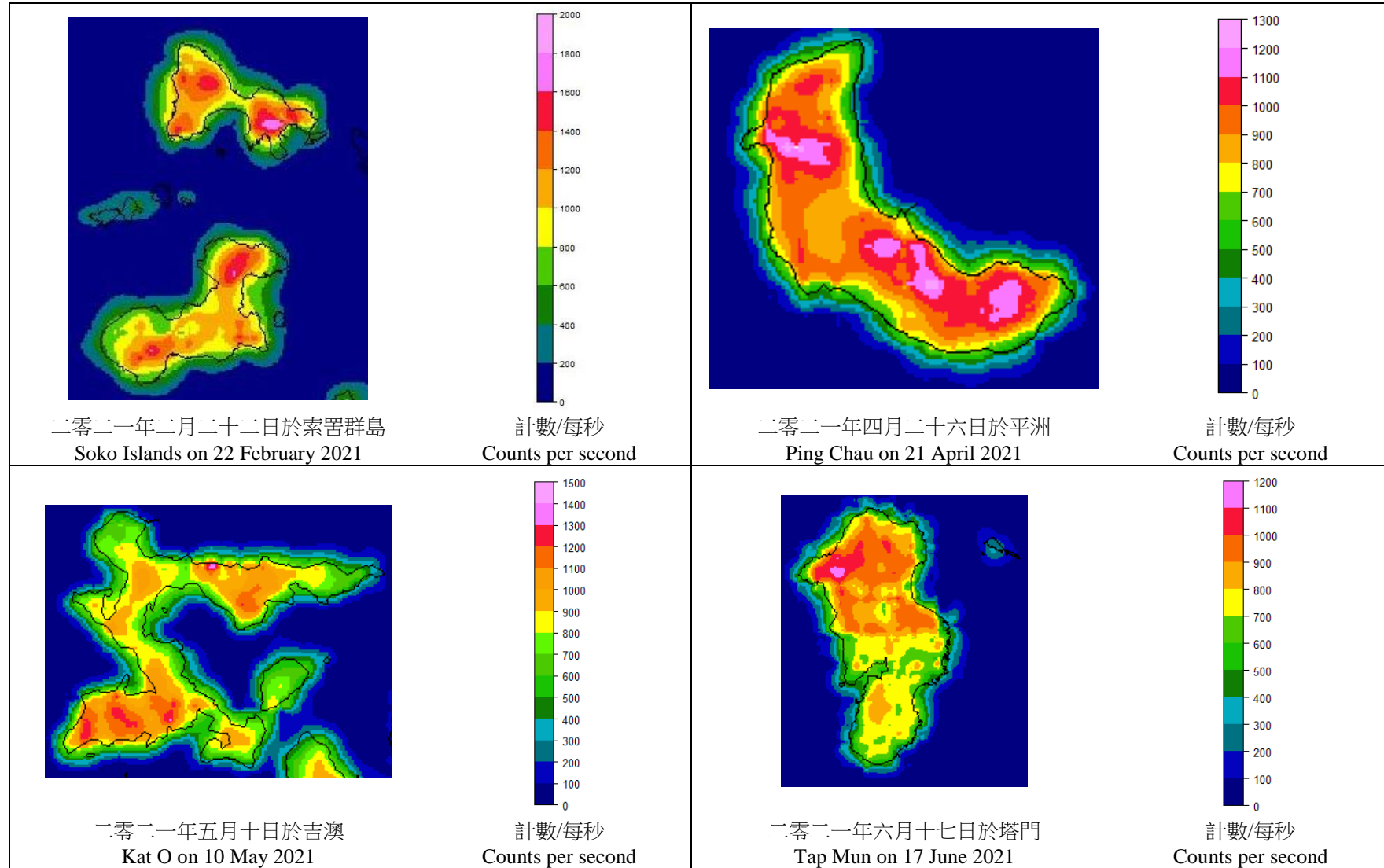
圖 4. 空中輻射監測系統在二零二一年分別於索罟群島、平洲、吉澳和塔門測量的計數率(測量高度距離地面約一百米)。 Figure 4. Count rate over Soko Islands, Ping Chau, Kat O and Tap Mun respectively as measured by the Aerial Radiation Monitoring System in 2021 (at about 100 metres above the ground).
