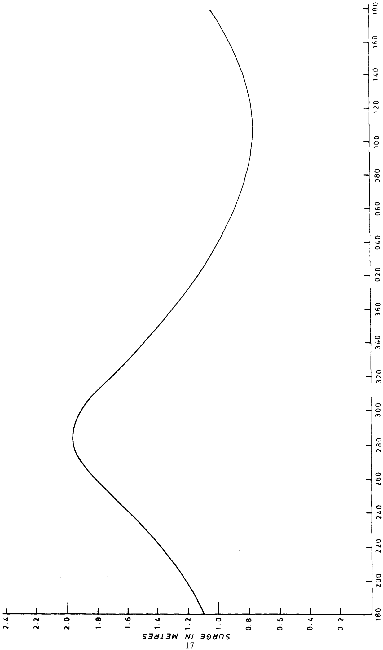
Figure 2. Splash nomogram – Splash computed North Point surge heights for various storm direction
