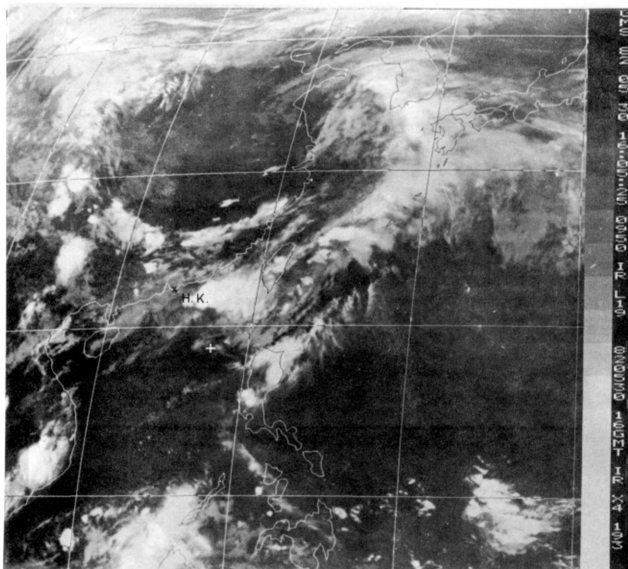
Plate 5. Infrared imagery taken at midnight, 30 May 1982
