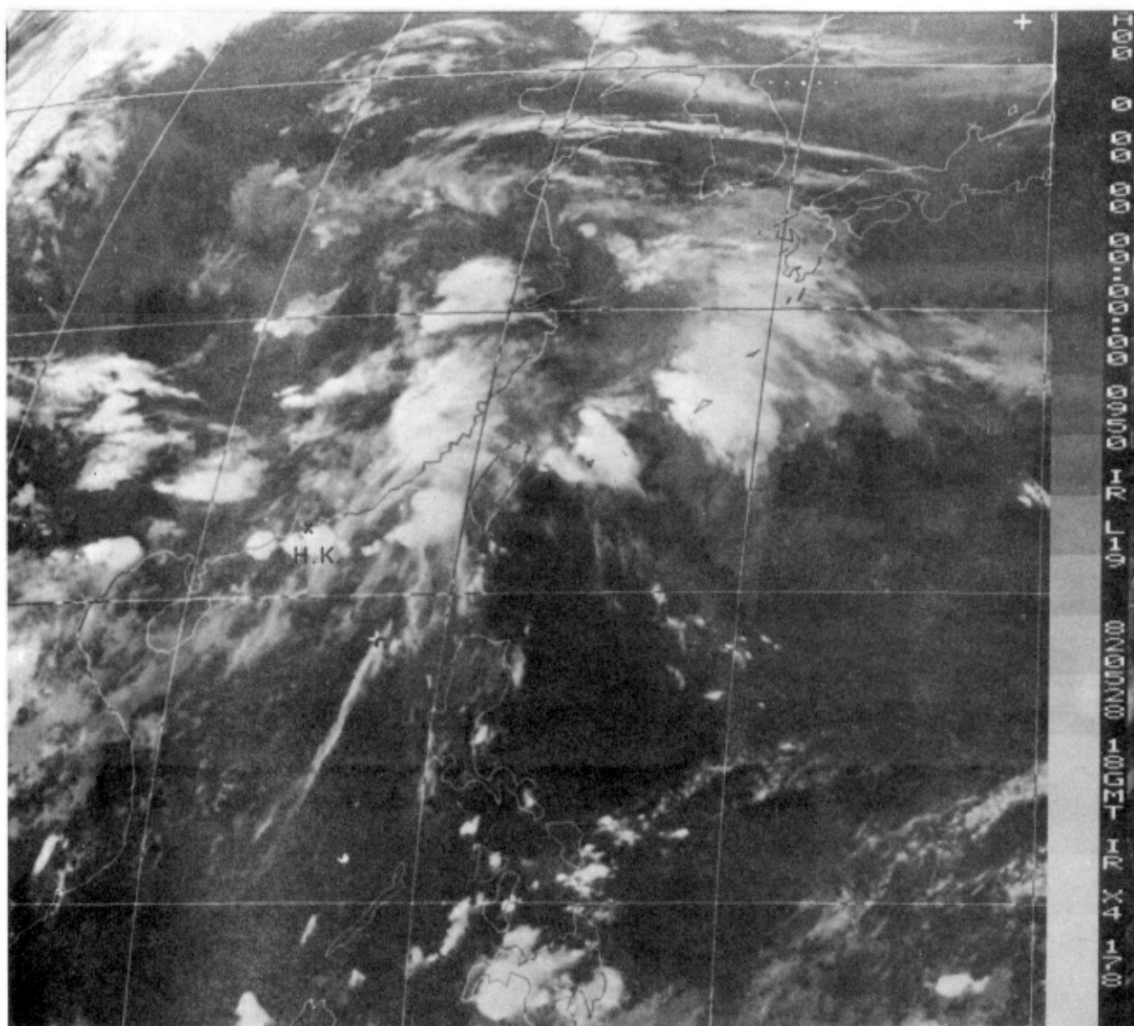
Plate 2. Infrared imagery taken at 2 a.m., 29 May 1982
