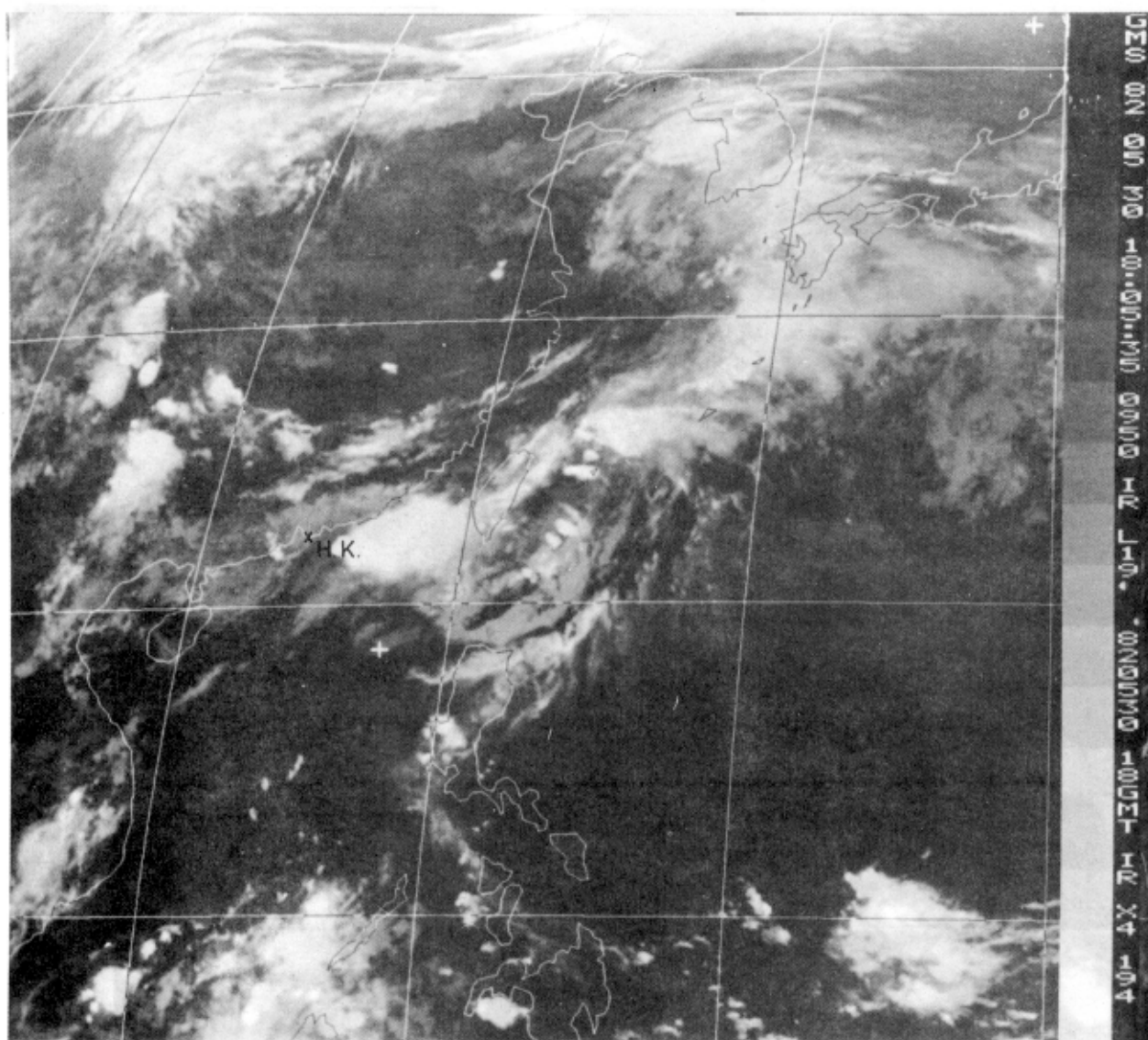
Plate 6. Infrared imagery taken at 2 a.m., 31 May 1982
