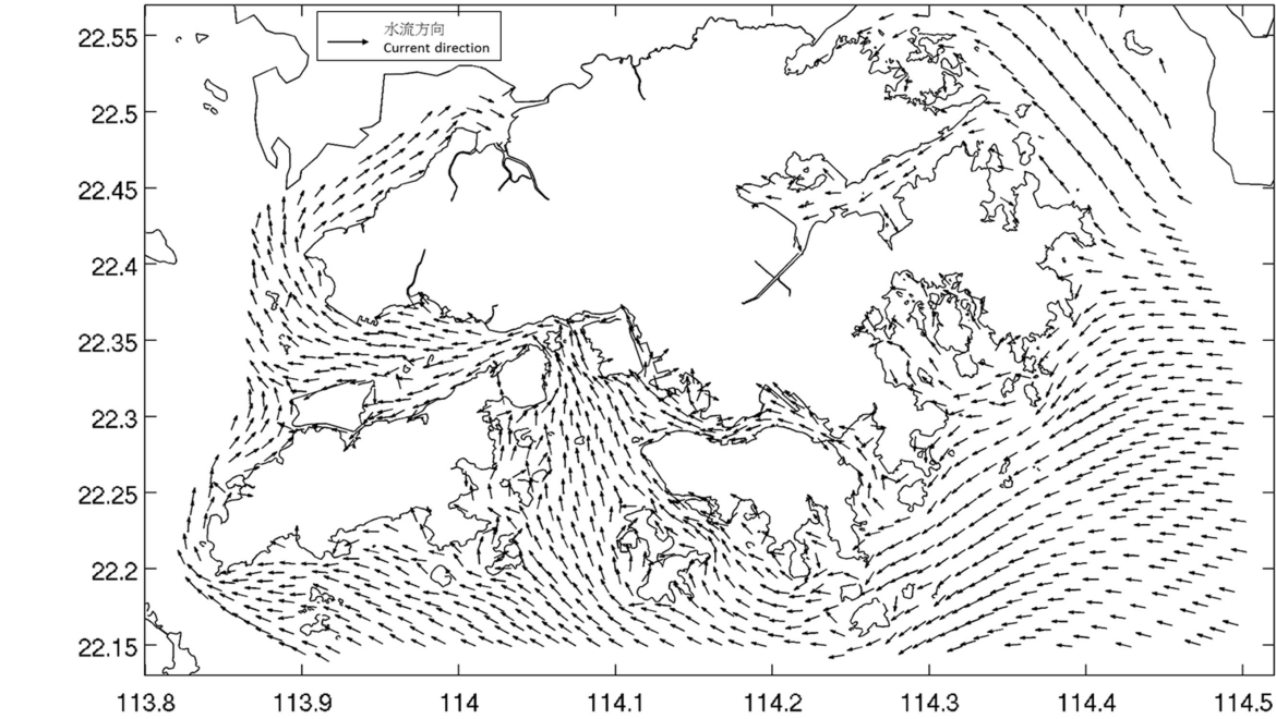
香港水域漲潮水流趨勢 Trend of tidal current in Hong Kong waters during flood tide
