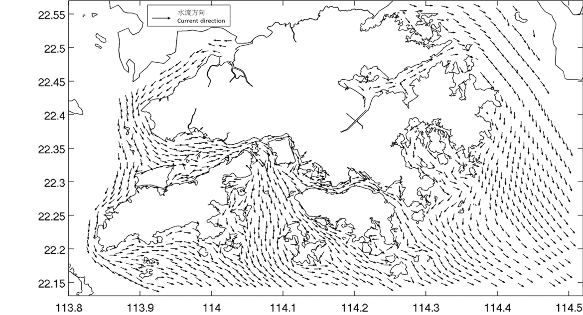
香港水域退潮水流趨勢 Trend of tidal current in Hong Kong waters during ebb tide
